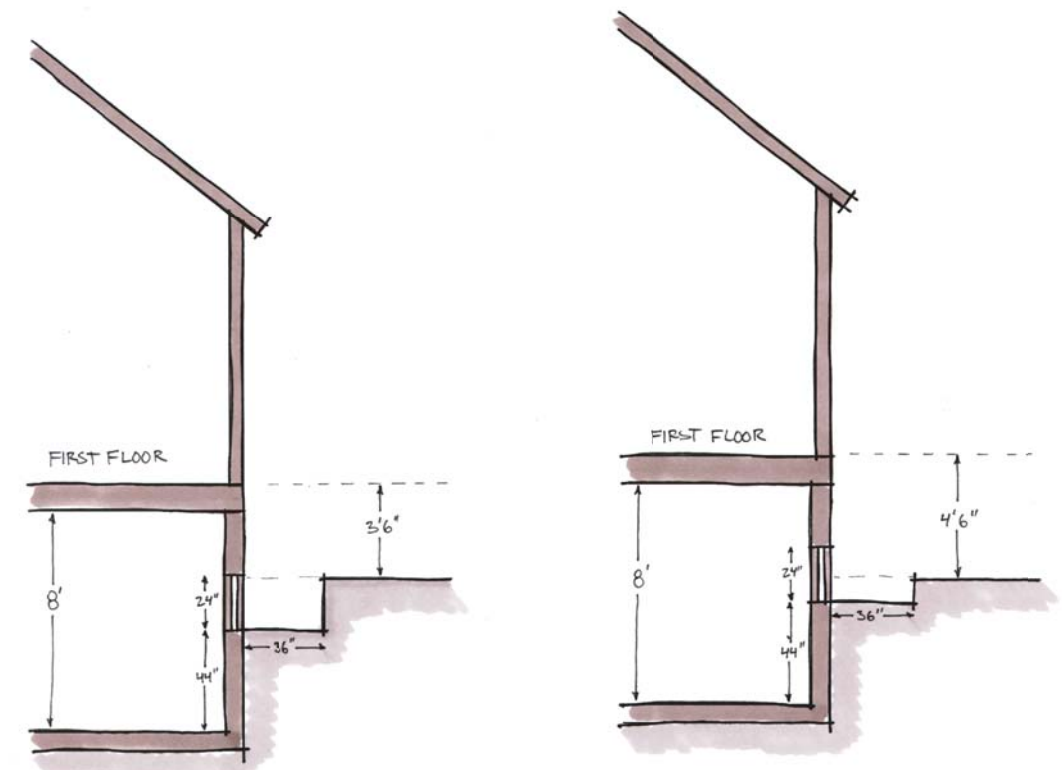
TYPICAL BASEMENT EGRESS
